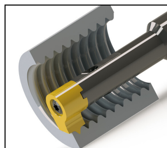
Single-point threading
