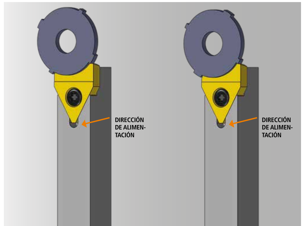
Placa intercambiable Schwanog 1 y placa intercambiable Schwanog 2
